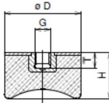
Gleiche Abmessungen wie DS-Puffer/ Same dimensions as DS-Bumpers
