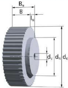
Stock pulleys over z = 48 without flanges
